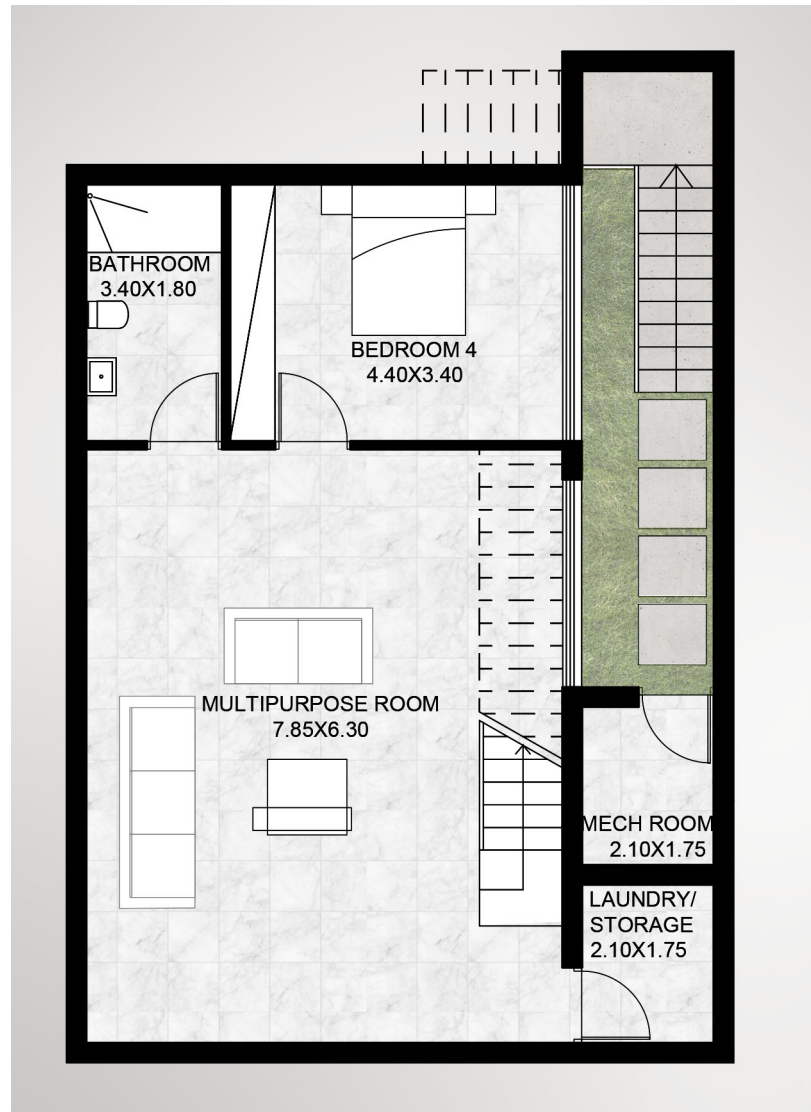
BASEMENT PLAN
